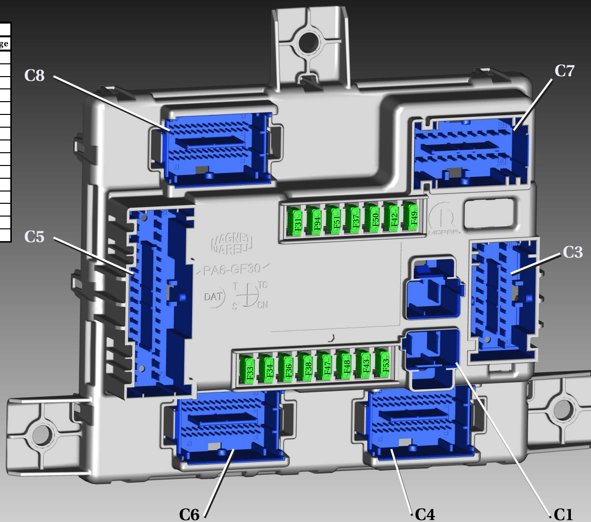
Body Contol Module (BCM)
